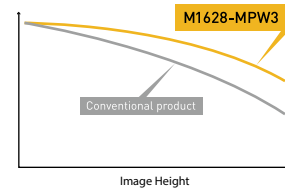
Relative Illumination
