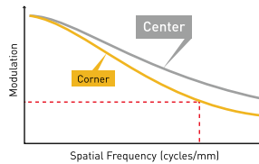
Conventional Product MTF WD300mm
