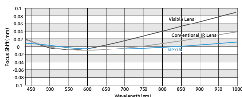
Chromatic Focus Shift
