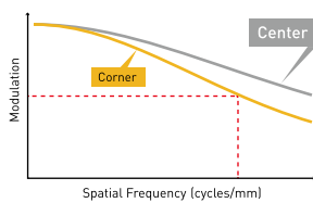
M1628-MPW3 MTF WD300mm
